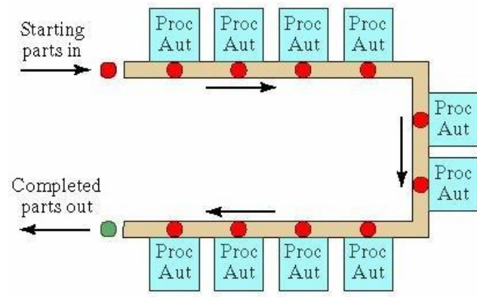
Figure 1.33 U-shaped configuration
