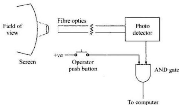
Figure 2.8 Light pen
