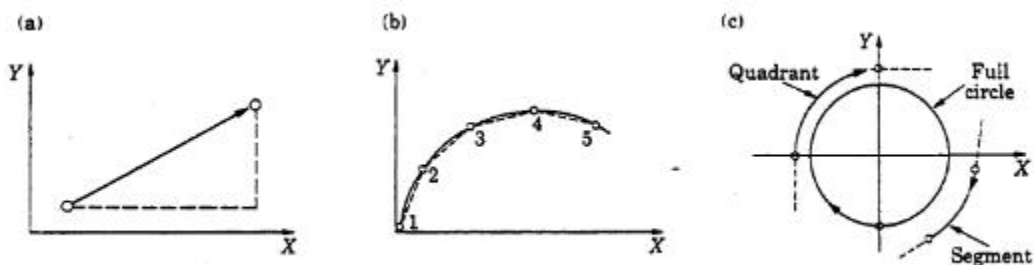
Figure 3.6 Interpolators
