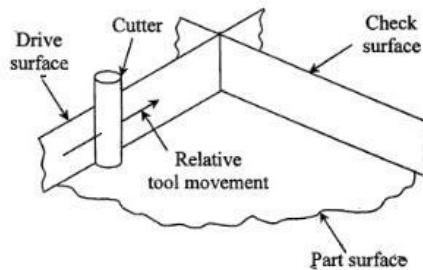
Three surfaces in APT contouring motions which guide the cutting tool
