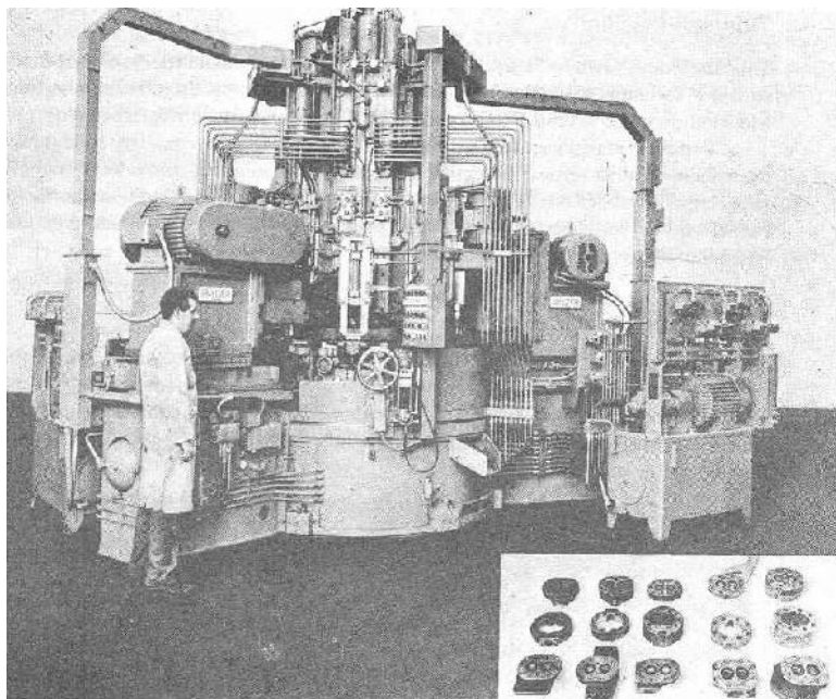
Figure 1.28 Ten-station center column machine
