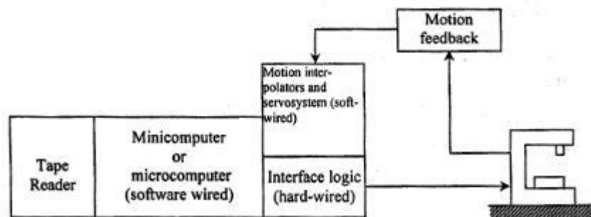
Figure 3.14 Hybrid CNC
