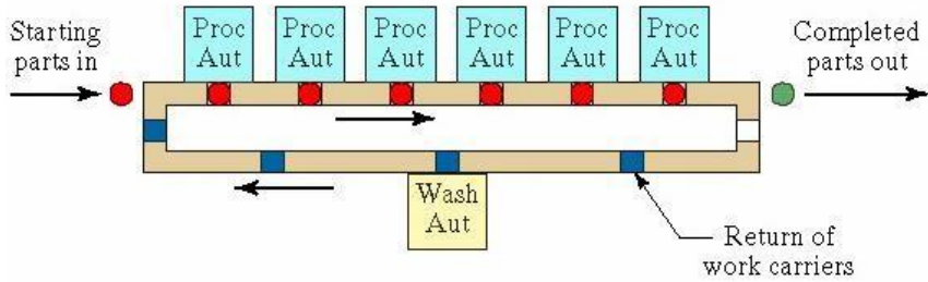
Figure 1.34 Rectangular-shaped configuration
