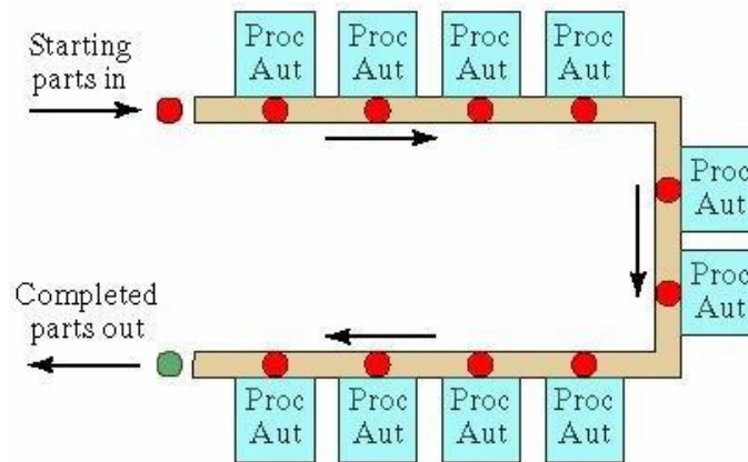
Figure 1.13 U-shaped configuration
