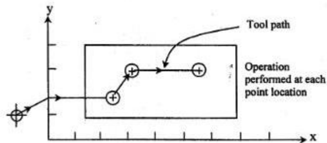
Figure 3.3 Point-to-point (positioning) NC system
