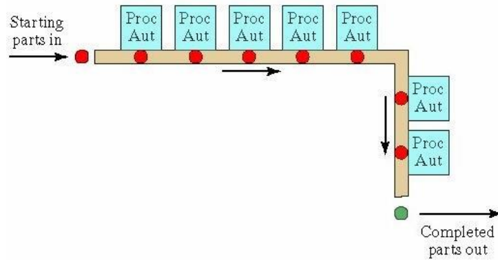
Figure 1.12 L-shaped configuration
