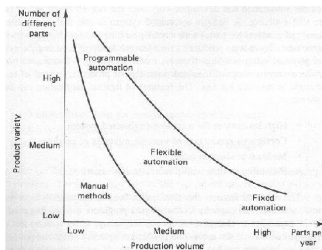
Figure 1.5 Types of automation as a function of volume of production versus product variety
