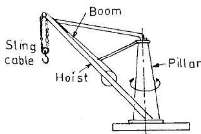
Fig. 4 Pillar Crane
