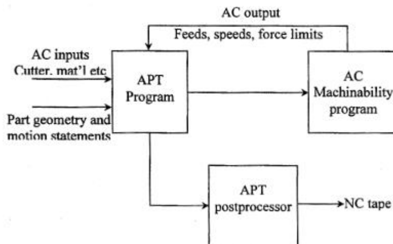
Figure 3.20 Relationship of adaptive control (AC) software to APT program
