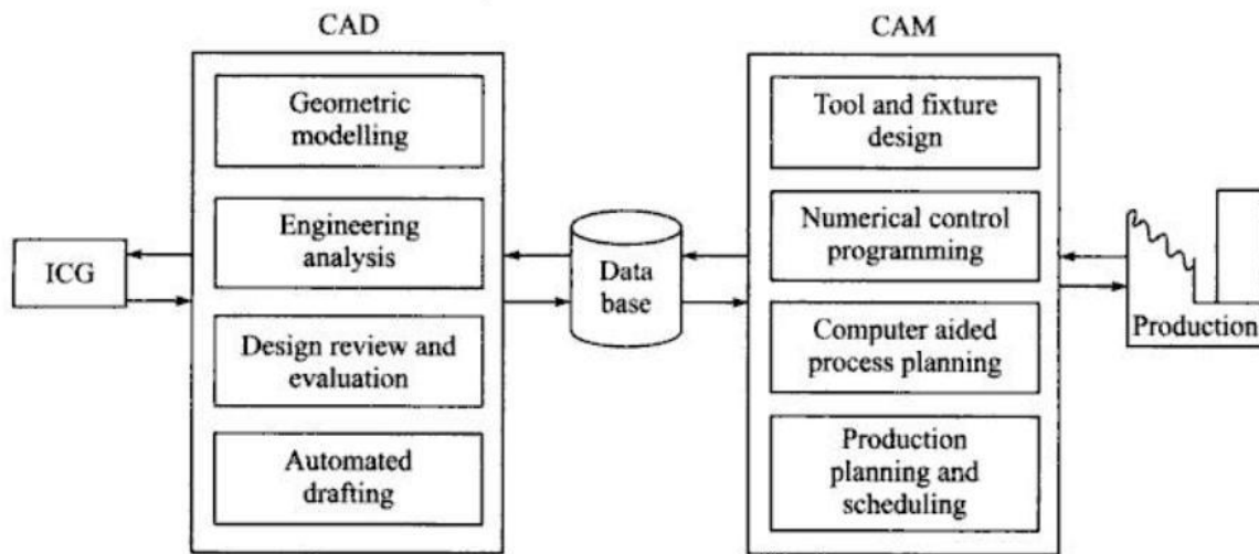
Figure 2.2 Relationship of CAD/CAM database to CAD and CAM
