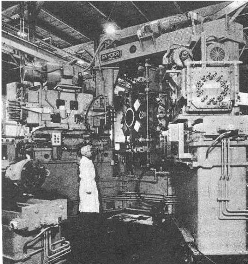
Figure 1.27 Six station trunnion machine
