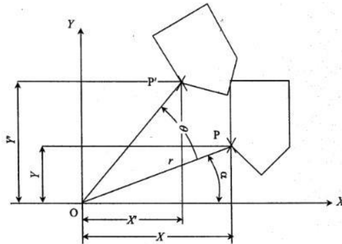
Figure 2.16 Rotation transformation
